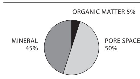
FIGURE 2. SOIL COMPOSITION: AN IDEALIZED SOIL
